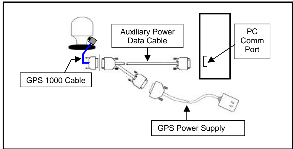
Figure 6. Antenna to PC cable connection
