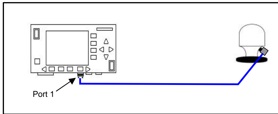
Figure 4. Cable attachment for PF3000 and GPS 1000
